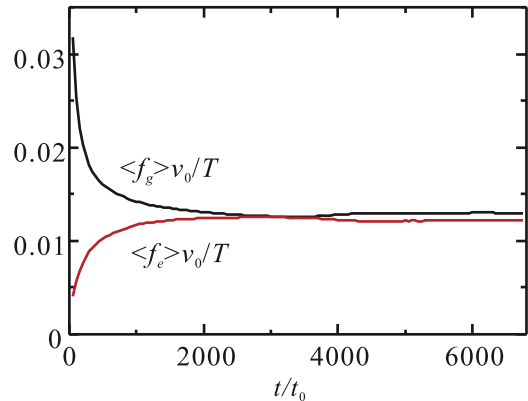
Figure 10. Space averages of f_g v_0/T and f_e v_0/T versus time t for n_e v_0 = 0.0025 , where \chi = 2.5 and \langle\phi\rangle = 1/2 .
